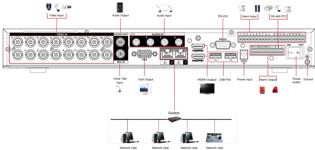
Figure 4-1 Connection diagram
